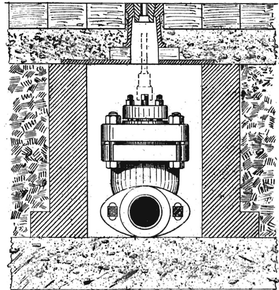
SECTION TRANSVERSE
