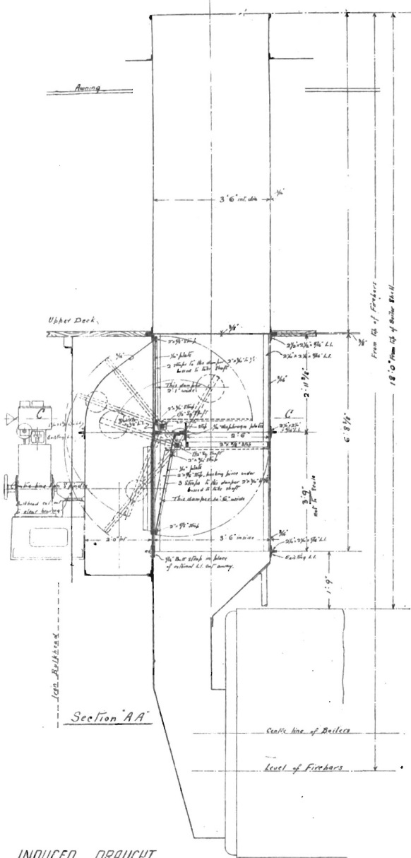
INDUCED DRAUGHT ARRANGEMENT
