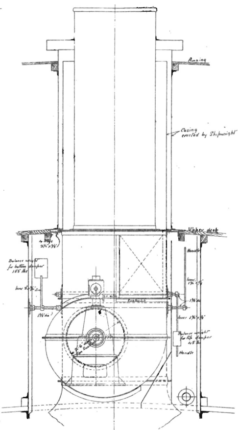
Section "BB"
