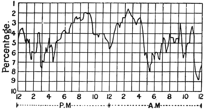
FIG. 1.—BOILER No. 29, FORCED DRAUGHT, HAND FIRED, No. 2 BUCKWHEAT COAL.
