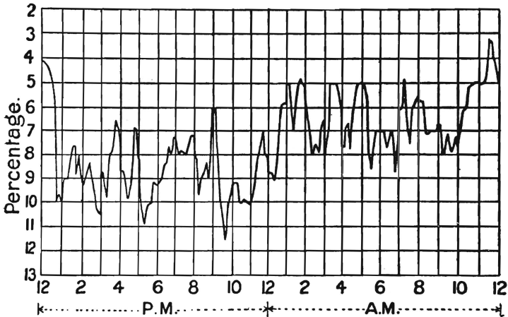
FIG. 2.—BOILER No. 29. UNDER SAME CONDITIONS AS FIG. 1, BUT WITH CAREFUL FIRING.
