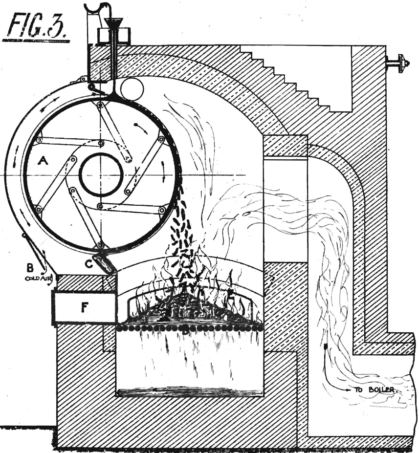
• DIAGRAMMATIC SKETCH • • ILLUSTRATING THE WORKING OF REVOLVING • • DRUM TYPE MOLASSES FURNACE. •
