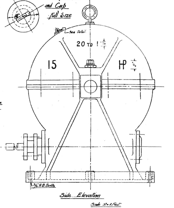
• 15 HP TWENTY TO ONE REDUCING BOX •
