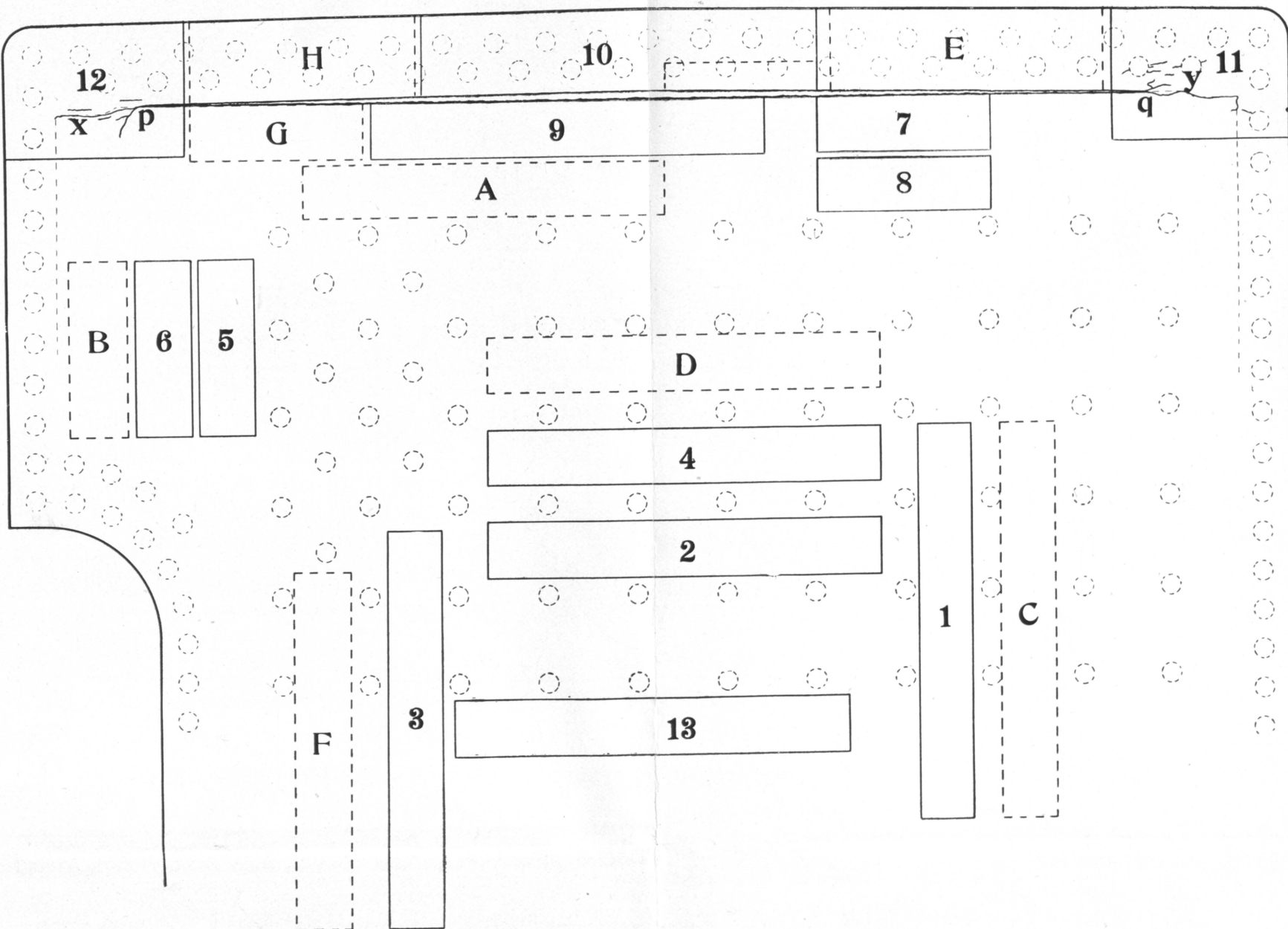
FIG. 2.—Diagram of Fractured Furnace Plate.
